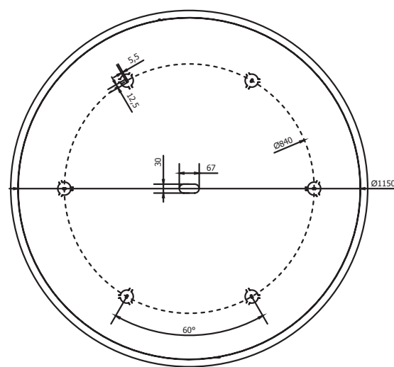
PIASTRA INTERNA / INTERNAL PLATE
